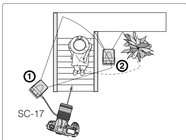
Wireless multiple flash (two flash units)
