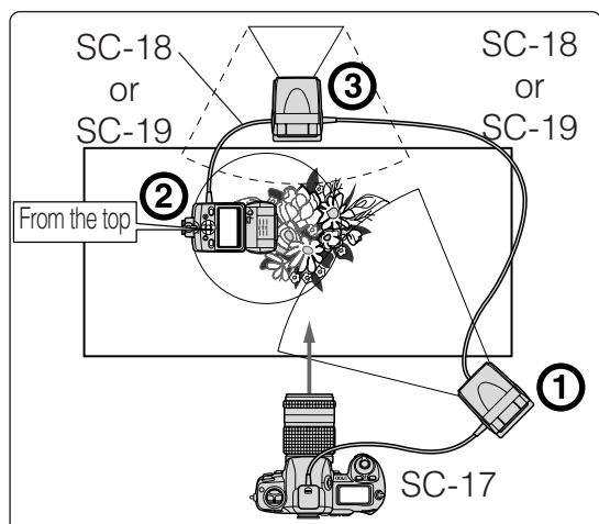
Multiple flash shooting (using 3 flash units)
