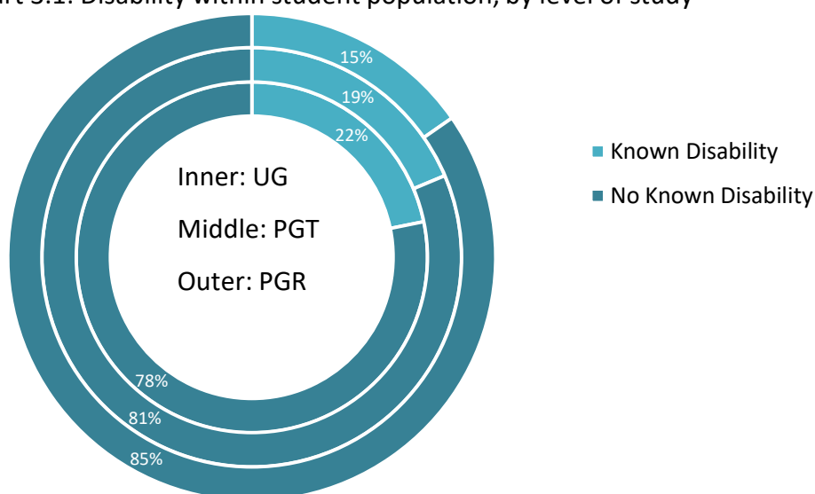
Chart 3.1: Disability within student population, by level of study
