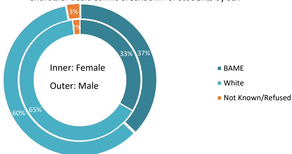
Chart 2.3: Basic ethnic breakdown of students by sex
