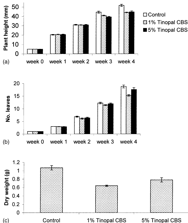
Fig. 3. Assessment of barley plants sprayed with 0, 1 or 5% Tinopal CBS over a 4-week period ( n = 20 per treatment): (a) mean height ( \pm S.E.); (b) mean number of leaves per plant ( \pm S.E.); (c) dry weight of aboveground foliage.
