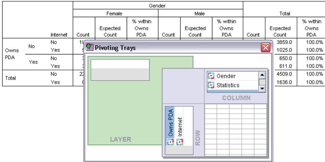
Figure 7-6 Swap rows
