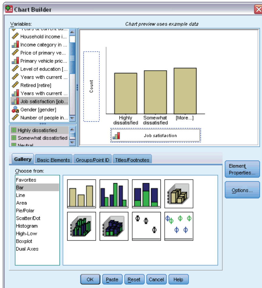
Figure 6-3
