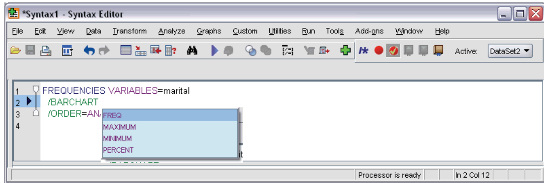
Figure 8-3
