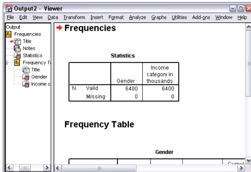
Figure 1-10 Viewer window
