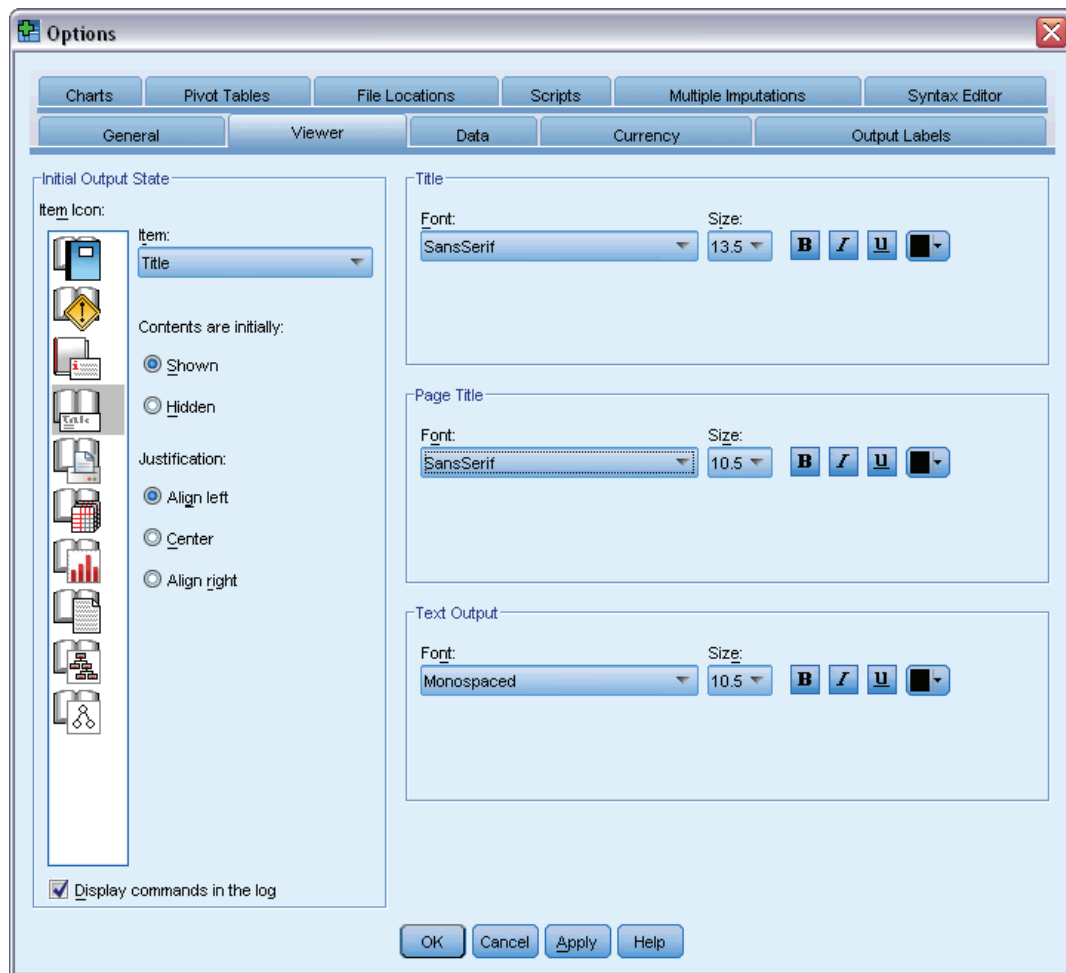
Figure 7-18 Viewer options
