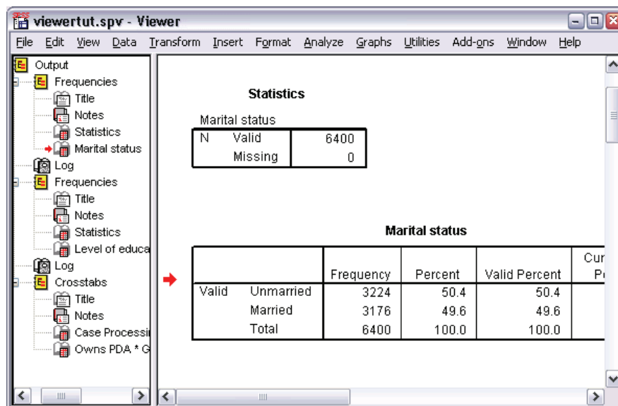
Figure 7-1 Viewer
