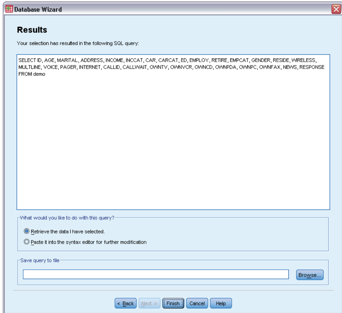
Figure 2-10 Results step
