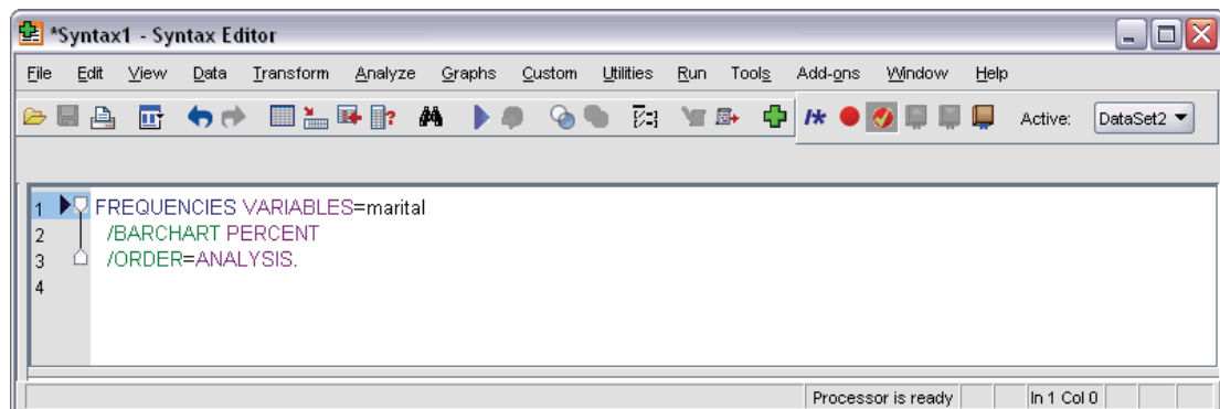
Figure 8-2 Frequencies syntax
