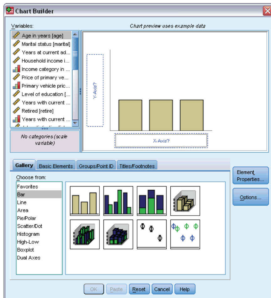
Figure 6-2
