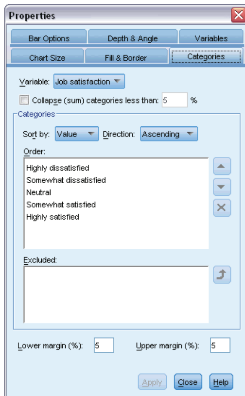
Figure 6-8 Properties window
