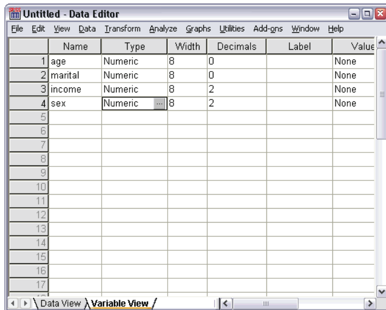
Figure 3-4
