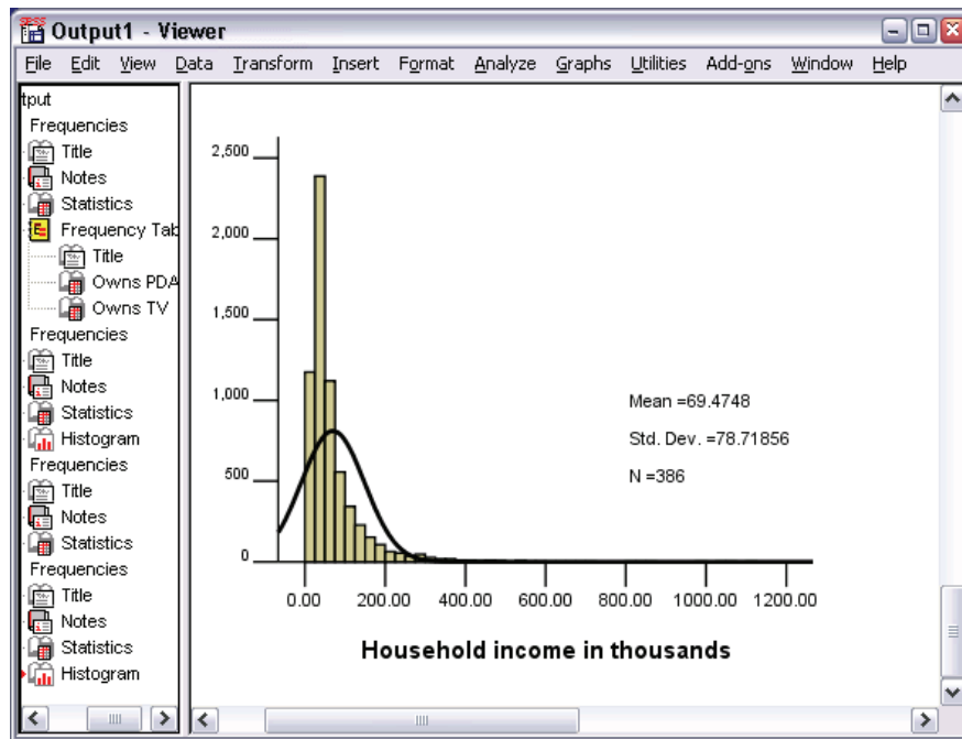
Figure 5-10 Histogram
