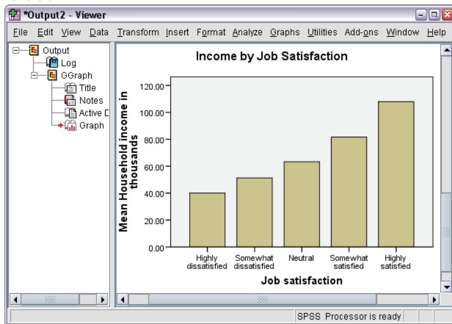
Figure 6-6 Bar chart
