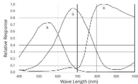
Spectral response of CoolCube 1c (color)
