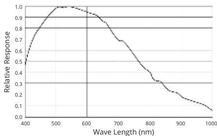
Spectral response of CoolCube 1m (monochrome)
