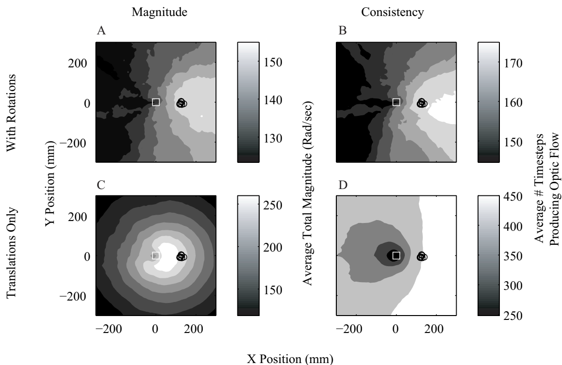
Fig. 4 Four different measures of optic flow. Combined data for 37 flights. A,B. Magnitude and consistency of optic flow for combined rotational and translational movements. C,D. Magnitude and consistency of optic flow for purely translational movements (see text for details). All distances are measured in mm. The nest (open square) is at (0,0) and the landmark (open circle) is at (125,0). Landmark positions varied slightly between recordings.
