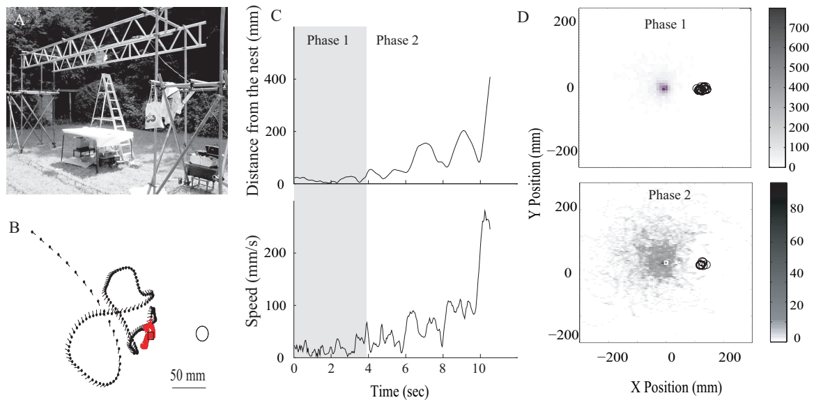
Fig. 2 A : A commercially available bumblebee hive is positioned underneath a featureless but textured 180\text{cm} \times 150\text{cm} board containing a single conspicuous landmark in the form of a small black cylinder. The bees enter and exit through an inconspicuous entrance that is positioned a small distance from the landmark. A camera was positioned on a frame and pointed down on the board in order to record the position and orientation of the bees during the initial phase of their foraging trips. B : An example of a bumblebee flight recorded with this set-up. The ball and stick icons represent the head position and body axis of the bee at 20ms intervals. The black circle represents the position of the 5cm diameter landmark. All distances are measured in mm. The nest (open square) is at (0,0) and the landmark (open circle) is at (125,0). C : The upper and lower traces represent the bee's distance away from the nest entrance and the bee's speed respectively. These parameters were used (see Methods) to determine the end of the first phase of bees' flights (red markers in B ). D Density plots showing the distribution of bee positions across all 37 flights for the first (top) and second (bottom) phases. The scale indicates the overall number of time-steps for which a bee was present at a given position in the ROI. The nest (open square) is at (0,0) and the landmarks (open circles) were at approximately (125,0). All distances are measured in mm.
