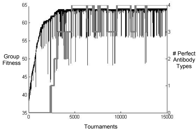
Figure 3: A plot of group fitness (black line) and number of antigens covered perfectly by at least one antibody (gray line) in the population over time for a single typical run of the 4 antigen task.
