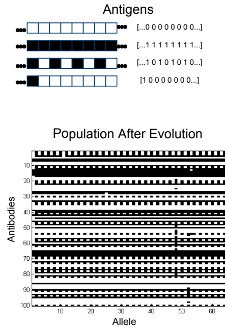
Figure 2: The antibody population after evolution on a 4 antigen task.
