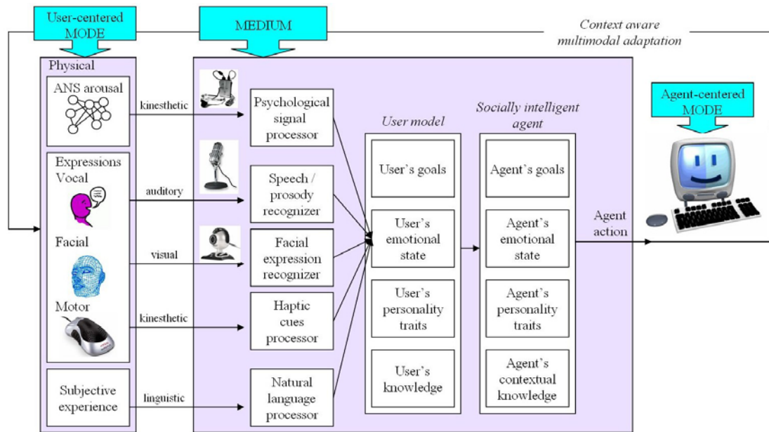
Figure 1: MAUI framework
