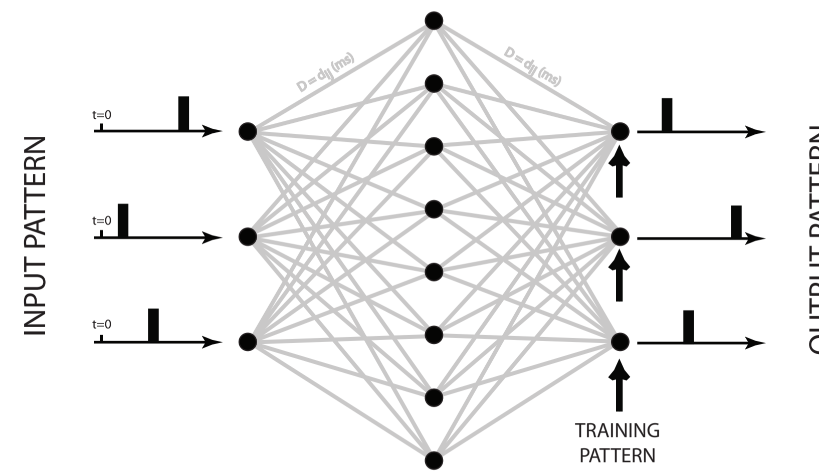
Figure 1: The Network Model
