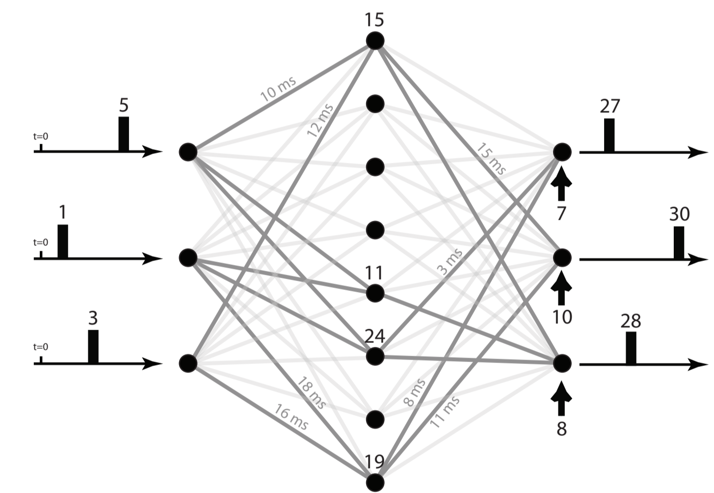
Figure 3: Learning spatiotemporal activity mappings with STDP and ITDP
