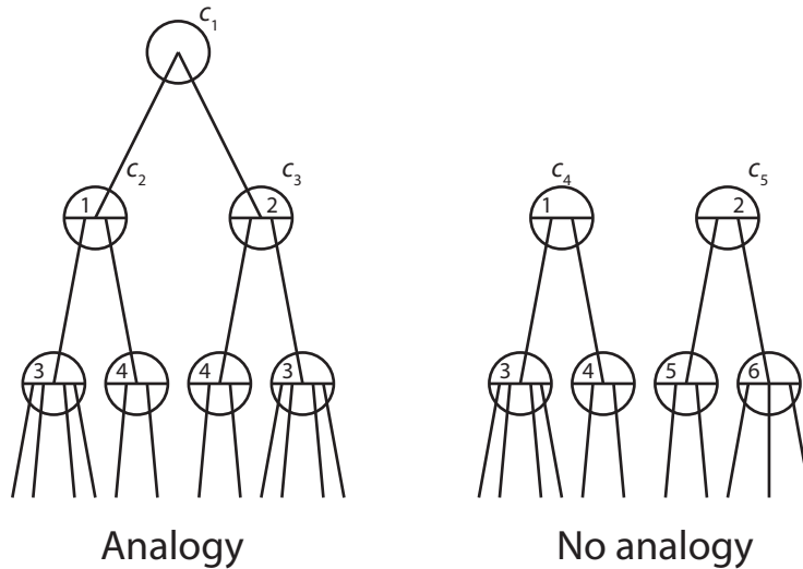
Figure 3: Formation of analogical mapping through conceptual-space exploration.
