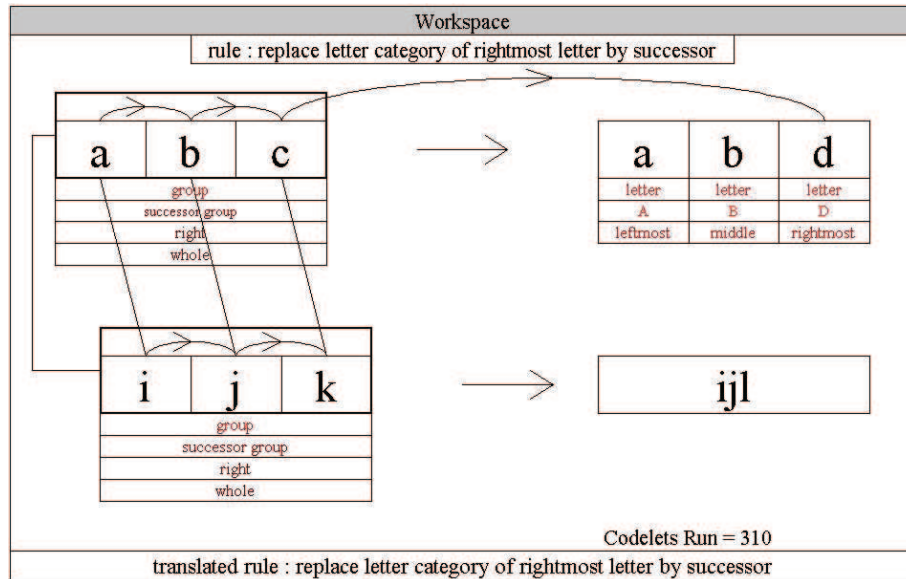
Figure 6: Construction of a letter-sequence analogy in Copycat.
