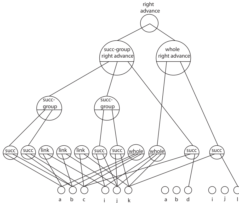
Figure 7: Copycat construction interpreted as conceptualization.
