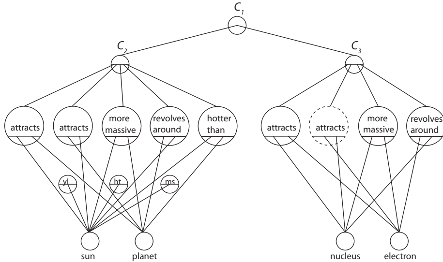
Figure 5: Transfer of relations in conceptual-space exploration (yl, ht and ms represent the properties of yellow, hot and massive here).
