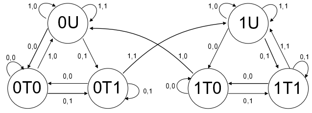
Figure 1. Directed graph of ETDL Moore FSM used to generate randomized test patterns.
