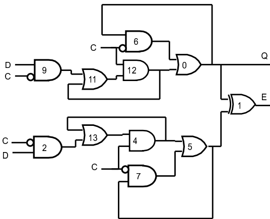
Figure 5. Evolved full on-line BIST solution for ETDL using 6 extra gates.
