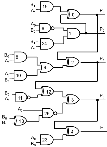
Figure 4. Evolved two bit multiplier with full on-line BIST using 9 extra gates.
